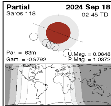
Five Millennium Canon of Lunar Eclipses (Espenak & Meeus) NASA TP-2009-214172
